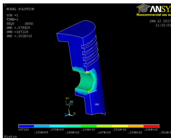
Figure 17: Equivalent stress (Von Mises Stress)
