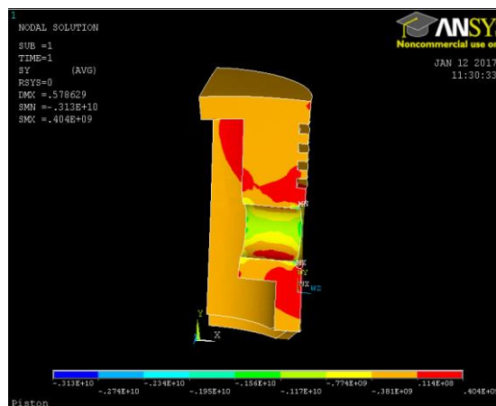
Figure 16: Stress (Y direction)
